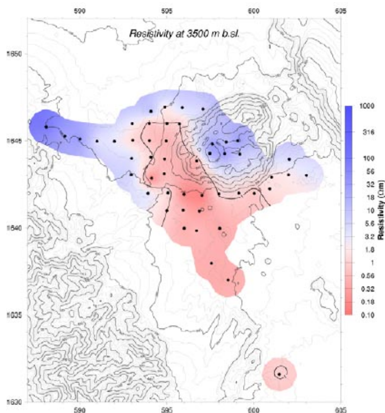
Figure 15: Resistivity map at 3500 m below sea level. Coordinates are in UTM, km units.
