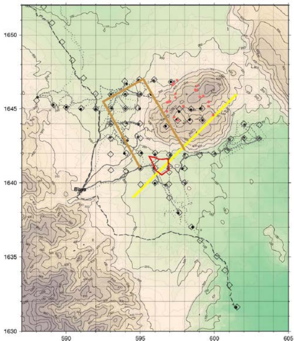
FIGURE 16: The yellow line shows the location of vertical resistivity boundary 0.5 and 2 km depth. The brown contour lines outline the low resistivity body west of Mt. Alid at about 2 km depth. Red dots are geothermal vents on Mt. Alid.
