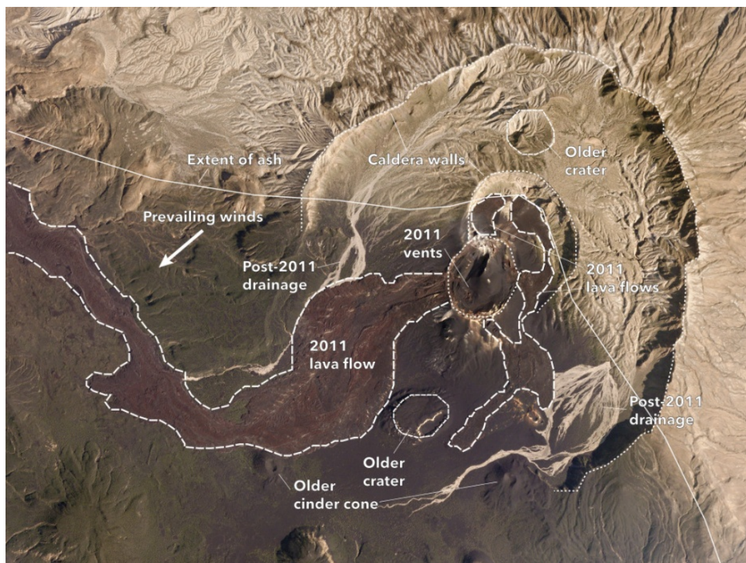
FIGURE 7: The 2011 volcanic eruption, both the trend of ash and flow
