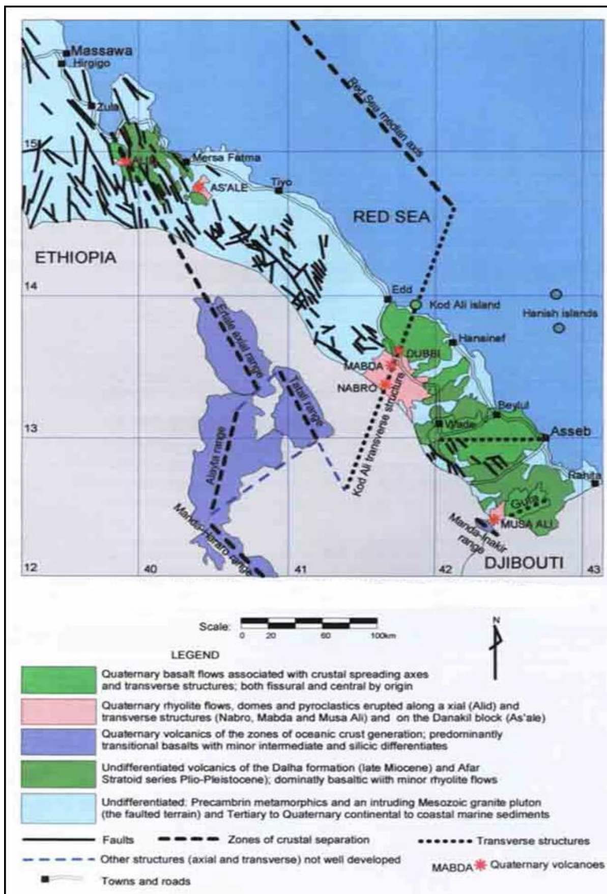
FIGURE 2: Regional geologic setting of the area
