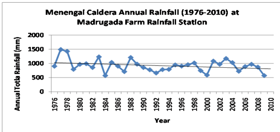
FIGURE 1: 1976 – 2010 Rainfall Madrugada farm, near Menengai caldera's edge (FOMECE, 2010)
