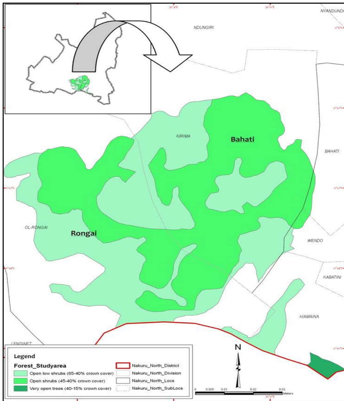
FIGURE 3: Vegetation distribution map of Menengai Caldera
