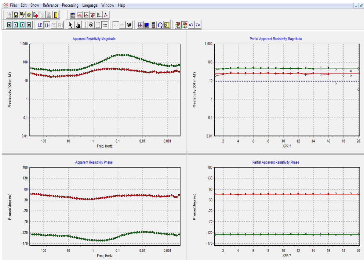
FIGURE 8: MT-editor frame
