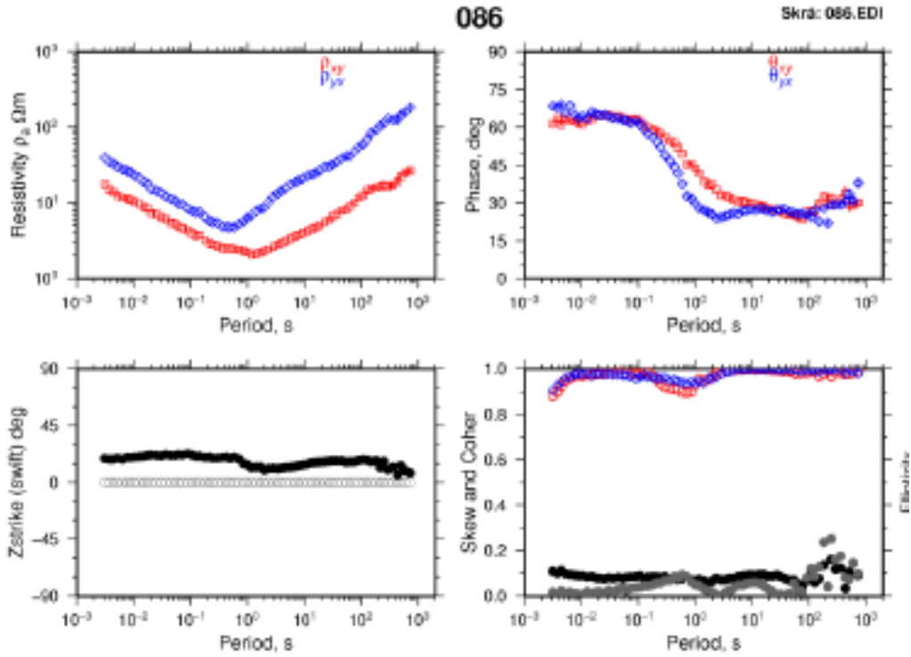
FIGURE 4: Apparent resistivity and phase, Z_{\text{strike}} , Skew and coherency for an MT sounding (taken from Hersir et al., 2009)
