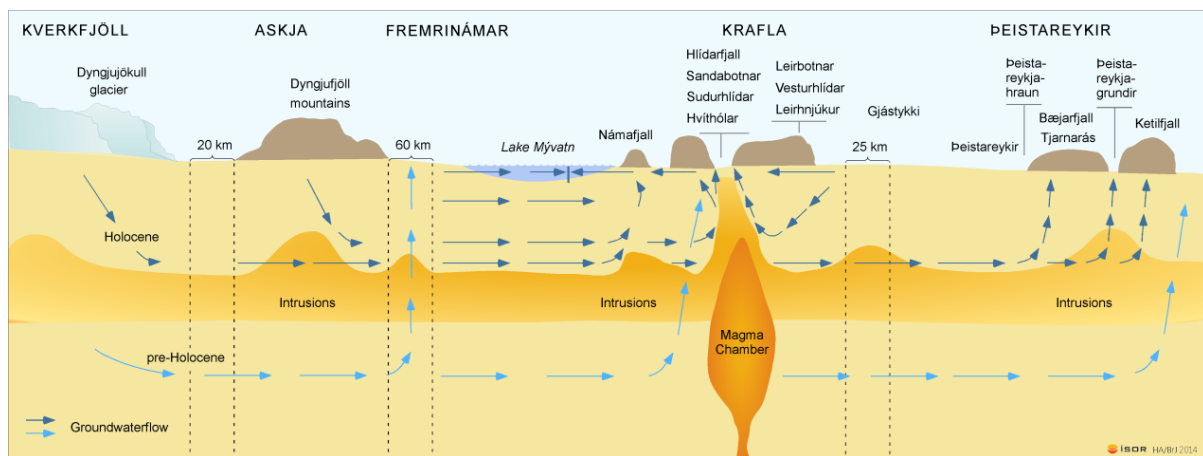
FIGURE 14: A conceptual hydrological model of the Northern Volcanic Zone. Modified from Hjartarson et al. (2004)
