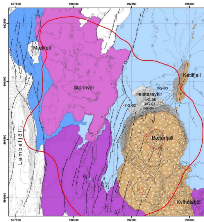
FIGURE 4: Size of the geothermal system according to results of resistivity soundings, 45 km 2 in total. The red line denotes the boundary of the high-resistivity core at 1 km depth. Wells marked PG are referred to with ThG in the text. From Saemundsson (2007).
