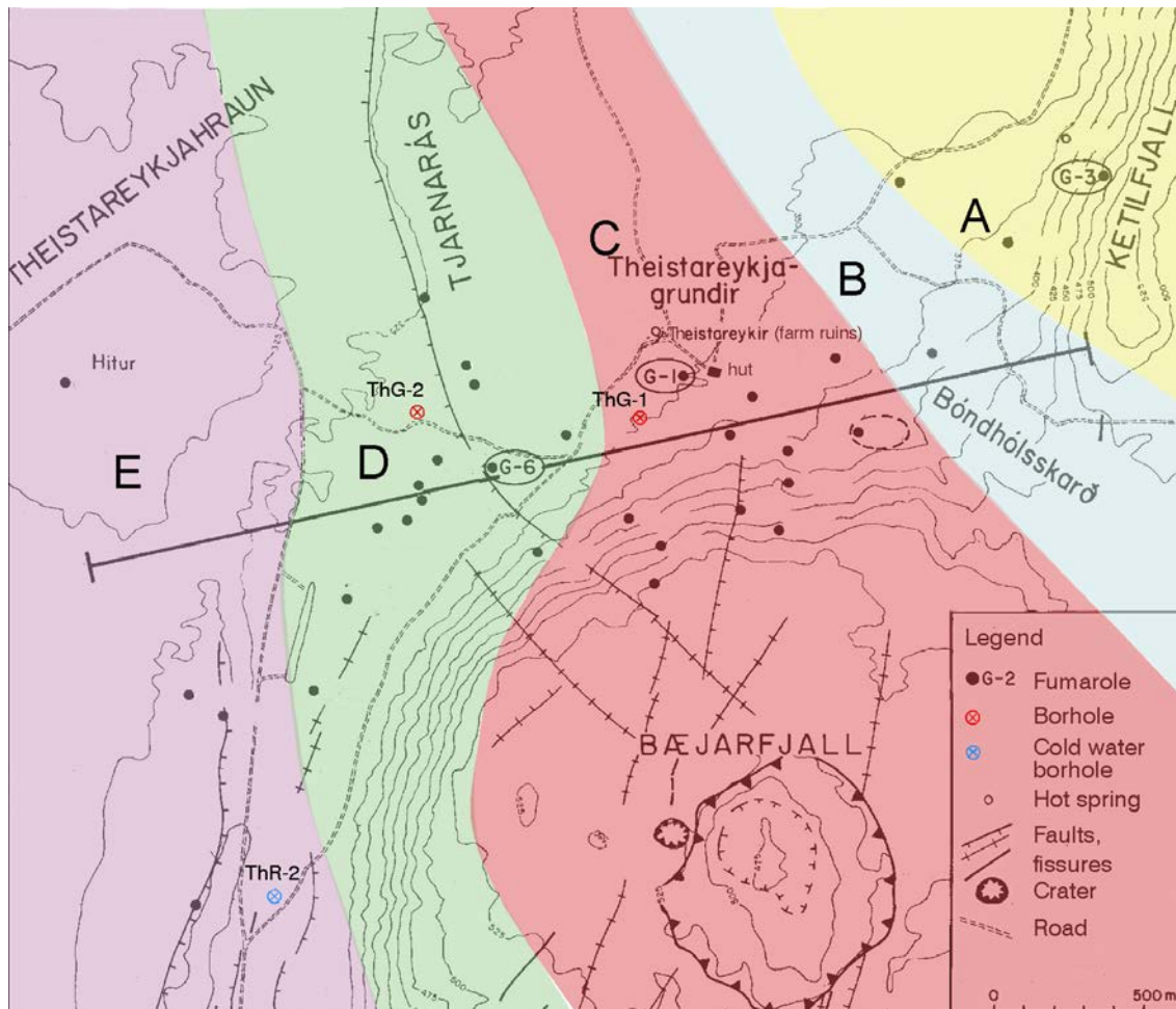
FIGURE 6: Division of the Theistareykir area into five sub-areas, based on chemical and isotope data (Ármansson et al., 1986)
