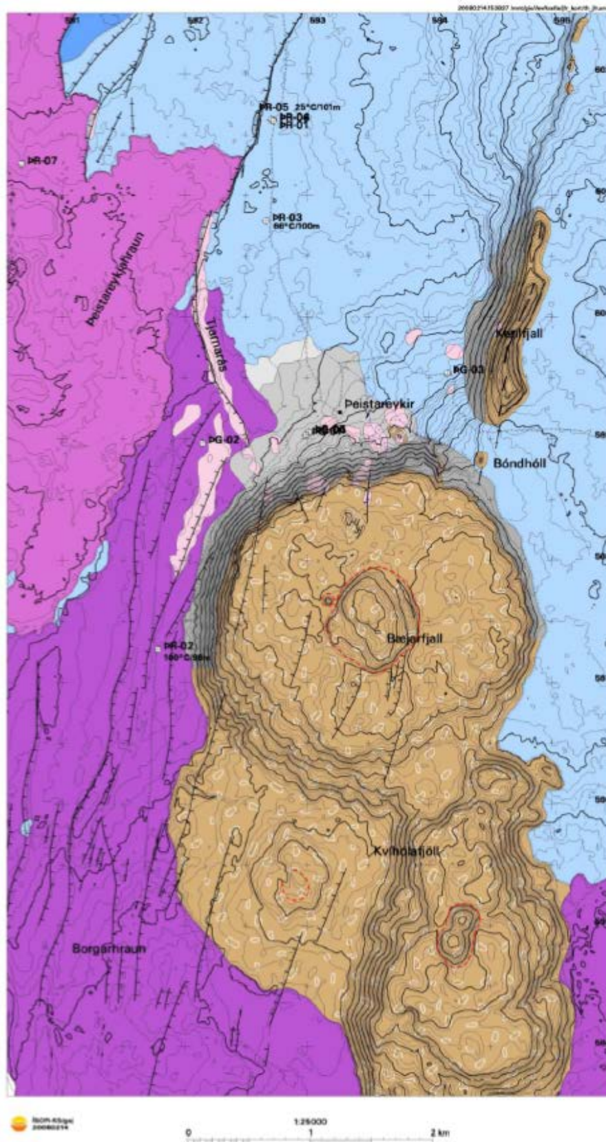
FIGURE 2: Geological map of Theistareykir. Hyaloclastites are brown, Borgarhraun dark purple, Theistareykjahraun light purple, Stórávítishraun light blue and Skildingahraun darker blue. Rock slides and surface deposits are grey. Wells marked PG on this and later figures are referred to with ThG in the text. From Sæmundsson (2007)
