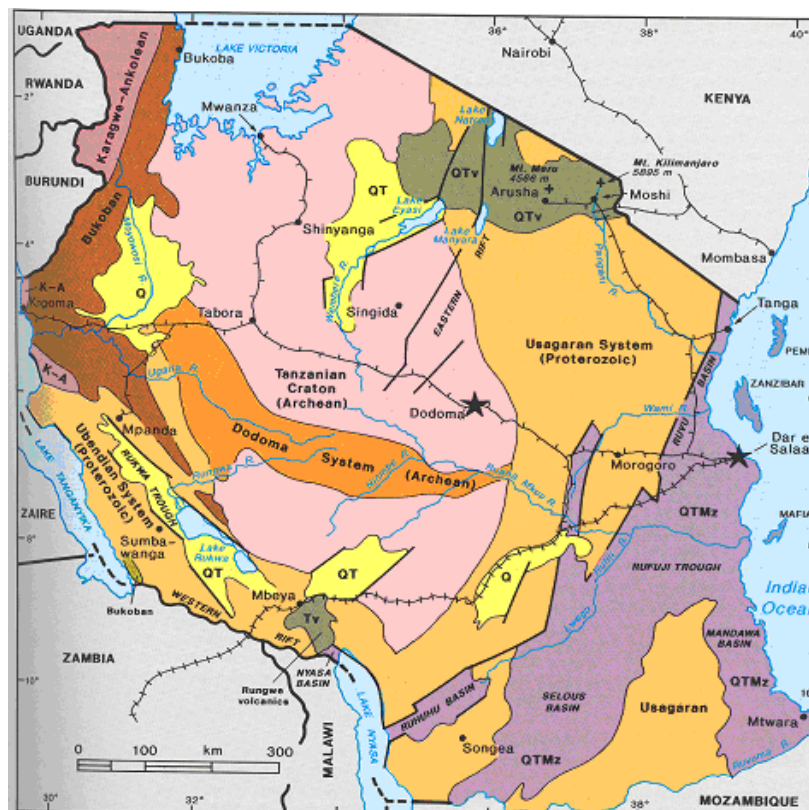
FIGURE 4: A simplified geological Map of Tanzania
