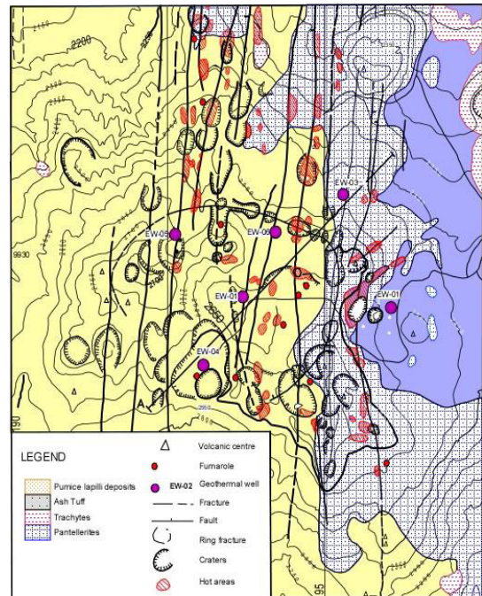
FIGURE 5: Map of Eburru geothermal field
