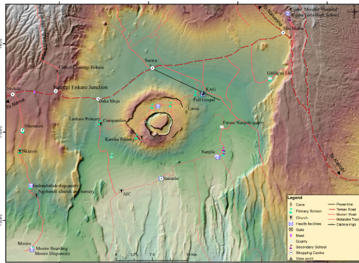
FIGURE 7: DEM image of Suswa geothermal prospect
