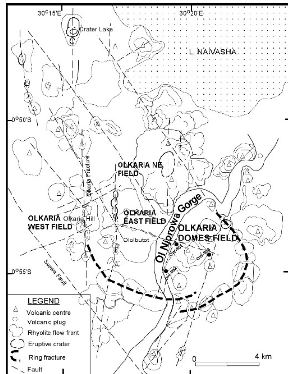
FIGURE 3: Structural map of Olkaria Geothermal
