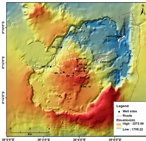
FIGURE 6: DEM image of Menengai
