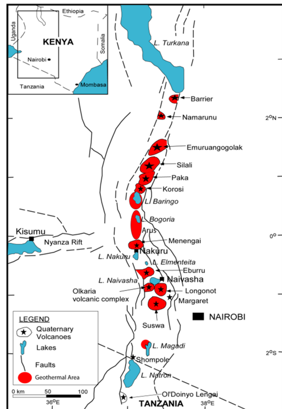
FIGURE 2: Simplified geological map of Kenya showing locations of the geothermal
