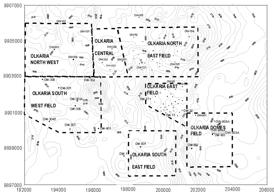
FIGURE 4: Map of the Greater Olkaria geothermal area
