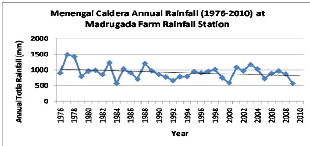
FIGURE 1: 1976 – 2010 Rainfall Madrugada farm, near Menengai caldera's edge (FOMECC, 2010)
