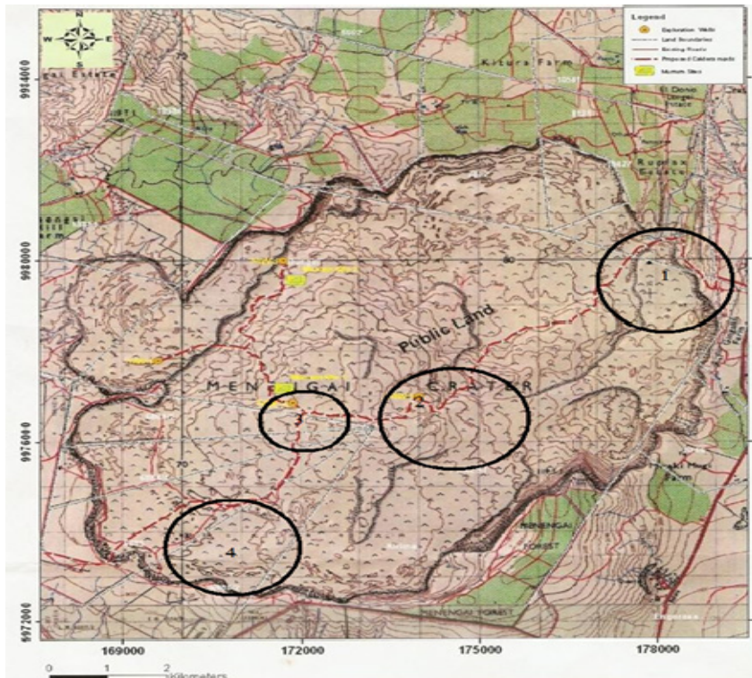
FIGURE 2: Study Area showing the plant sampling sites (modified from KenGen. 2008)
