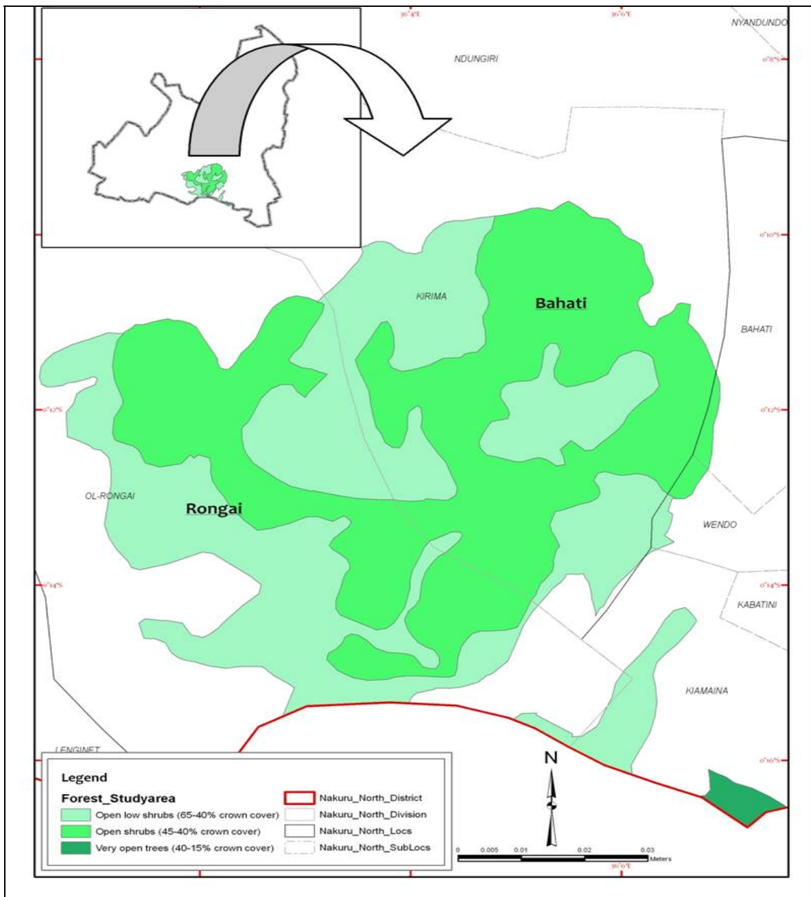
FIGURE 3: Vegetation distribution map of Menengai Caldera
