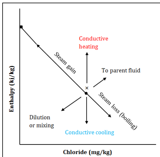
FIGURE 8: Chloride-enthalpy mixing model (modified after Nicholson, 1993)
