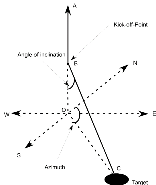
FIGURE 1: Measurement parameters of a directional well (modified from Gabolde and Nguyen, 1991)
