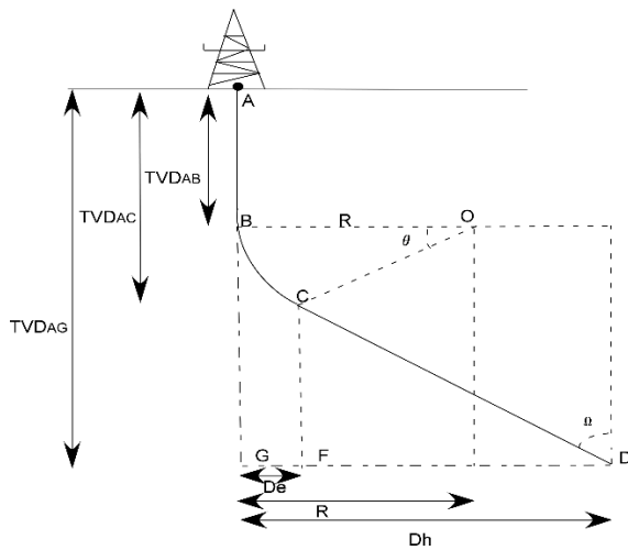
FIGURE 5: Geometry of build-and-hold type well path for D_h > R
