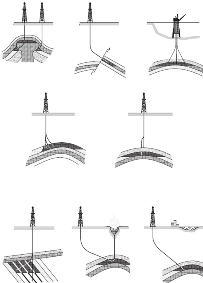
FIGURE 2: Several applications of directional drilling as common in the oil industry (Bourgoyne at al., 1991)
